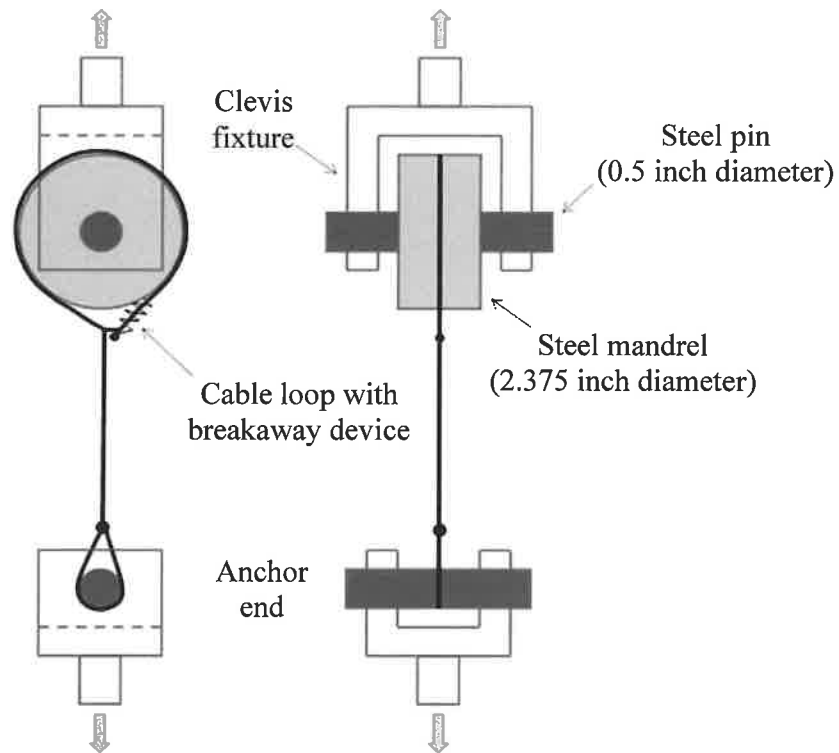
Figure 1: Test fixture, side and front views.
