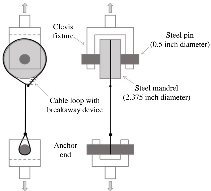
Figure 1: Test fixture, side and front views.
