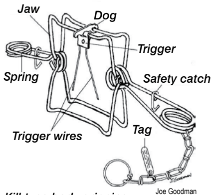
Kill-type body-gripping trap.
