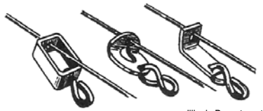
Submersion system locks.
