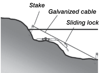
Submersion set. Silvertip Productions
