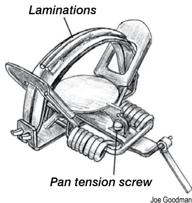
Laminated trap jaws. Joe Goodman
