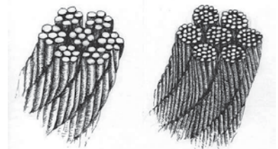
Natalene Cummings 7x7 Cable. 7x19 Cable.
