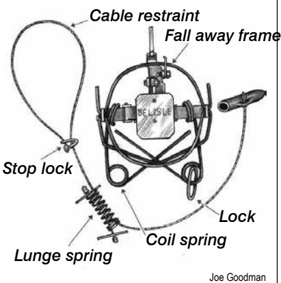
Unset spring-activated foothold cable device.
