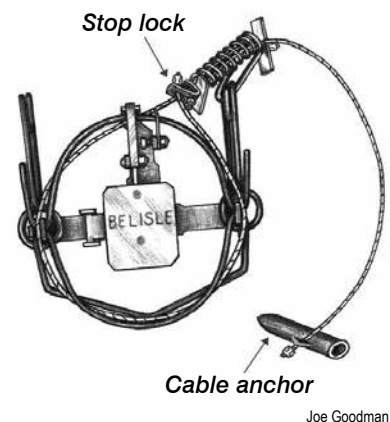
Coil-spring activated foothold cable device in the set position.
